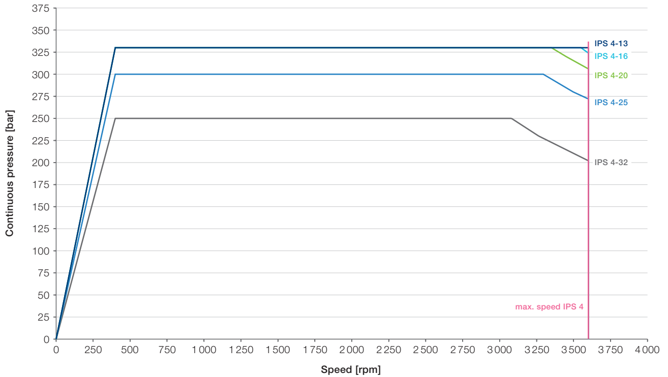
Diagram IPS 4 – Continuous pressure depending on the speed
